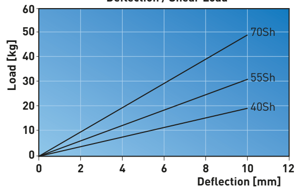
Deflection / Shear Load
