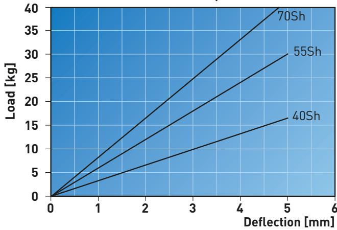
Deflection / Compression
