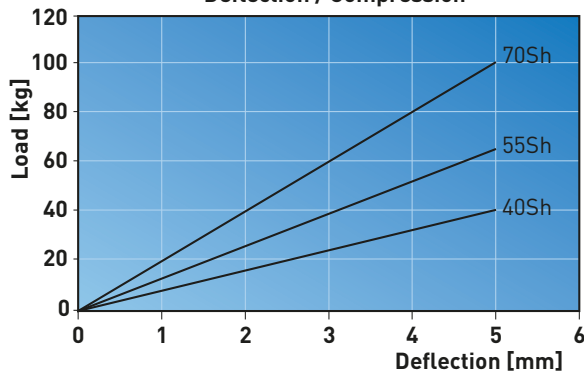
Deflection / Compression
