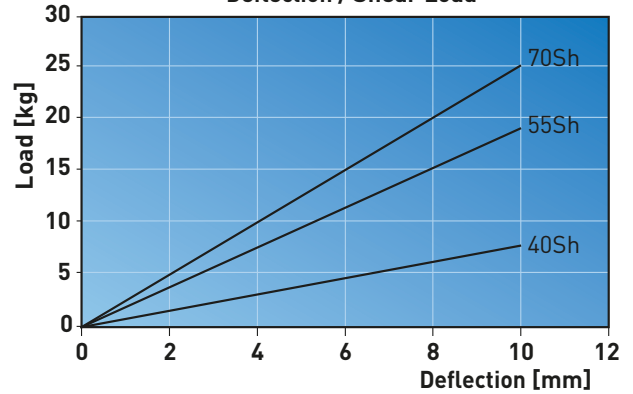
Deflection / Shear Load
